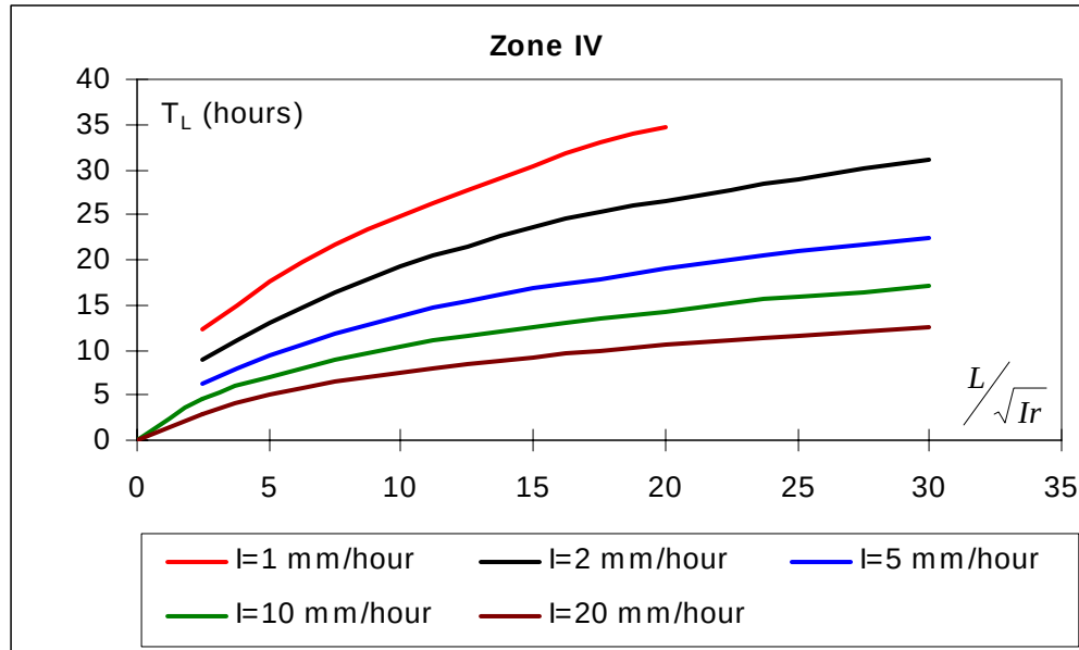
Figure 1. Regionalization relationships for the parameter T_L
